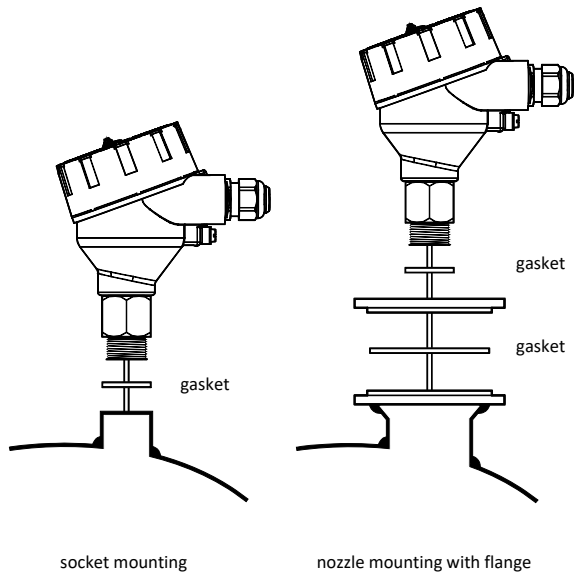
Figure 1: mounting
