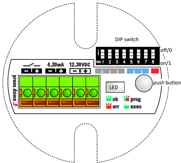
Figure 9: control elements
