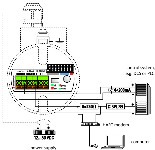
Figure 8: wiring
