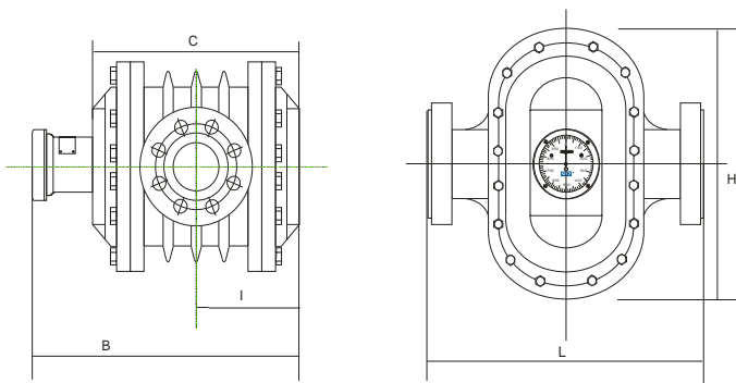
DN150-DN200
