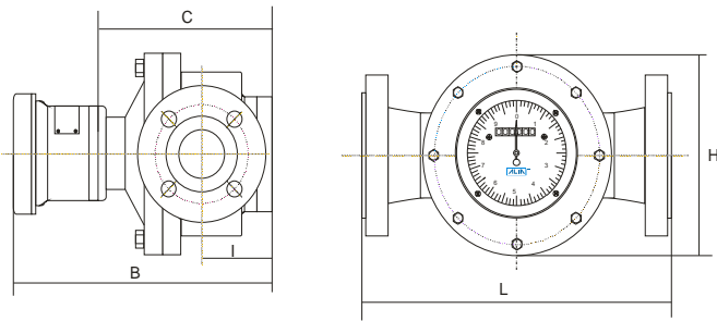
DN10-DN40
