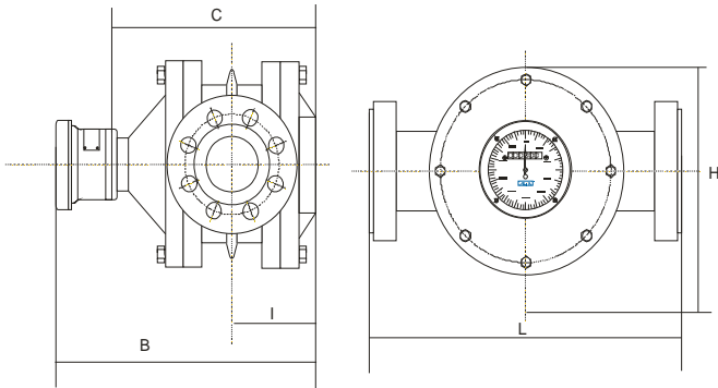
DN50-DN100
